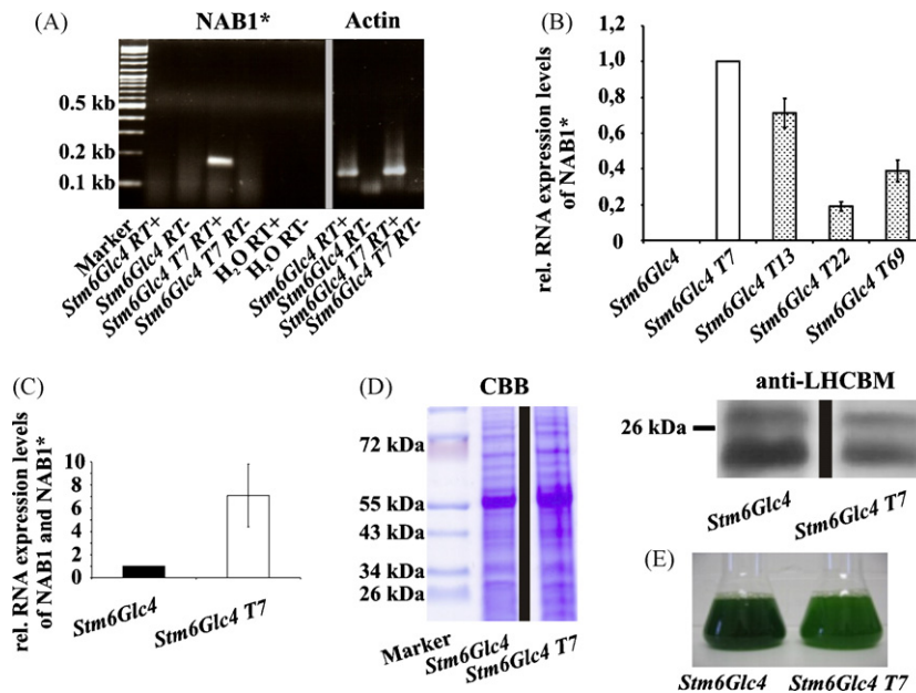
Fig. 2. Evidence for functional NAB1* expression in T7 and phenotypical analysis. (A) Analysis of NAB1* expression levels by RT-PCR. Signal detection was performed after 29 cycles using primer pair: qRT_3'NAB*1_fow (5'cgacaagttgaacaacagcc3'), qRT_3'NAB*1_rev (5'ccgctatcaatcagcgaa3'); product size: 150 bp. \beta -Actin was used as a control. (B) Comparative analysis of mutated NAB1* RNA expression levels by Q-RT-PCR in different mutant strains. The expression level of strain T7 was set to 1. (C) Quantification of the endogenous NAB1 and of the mutated NAB1* transcripts by Q-RT-PCR. The expression level of the parental strain Stm6Glc4 was set to 1. \beta -Actin transcript levels were used to normalize the NAB1 and NAB1* expression. (D) Immunoblot analysis using antibodies specific for all LHClI isoforms. Total protein extracts derived from Stm6Glc4 and T7 were separated by Tris-Tricine-SDS-PAGE (10% (w/v) acrylamide) and transferred to nitrocellulose membranes. Left panel: Coomassie blue stain (loading control), right panel: anti-LHClI immunoblot. (E) Appearance of T7 (right) and the parental strain Stm6Glc4 (left) after photoautotrophic growth in HSM medium to the late logarithmic phase. Cell cultures were adjusted to equal cell densities ( 1.75 \times 10^7 cells mL -1 ).
